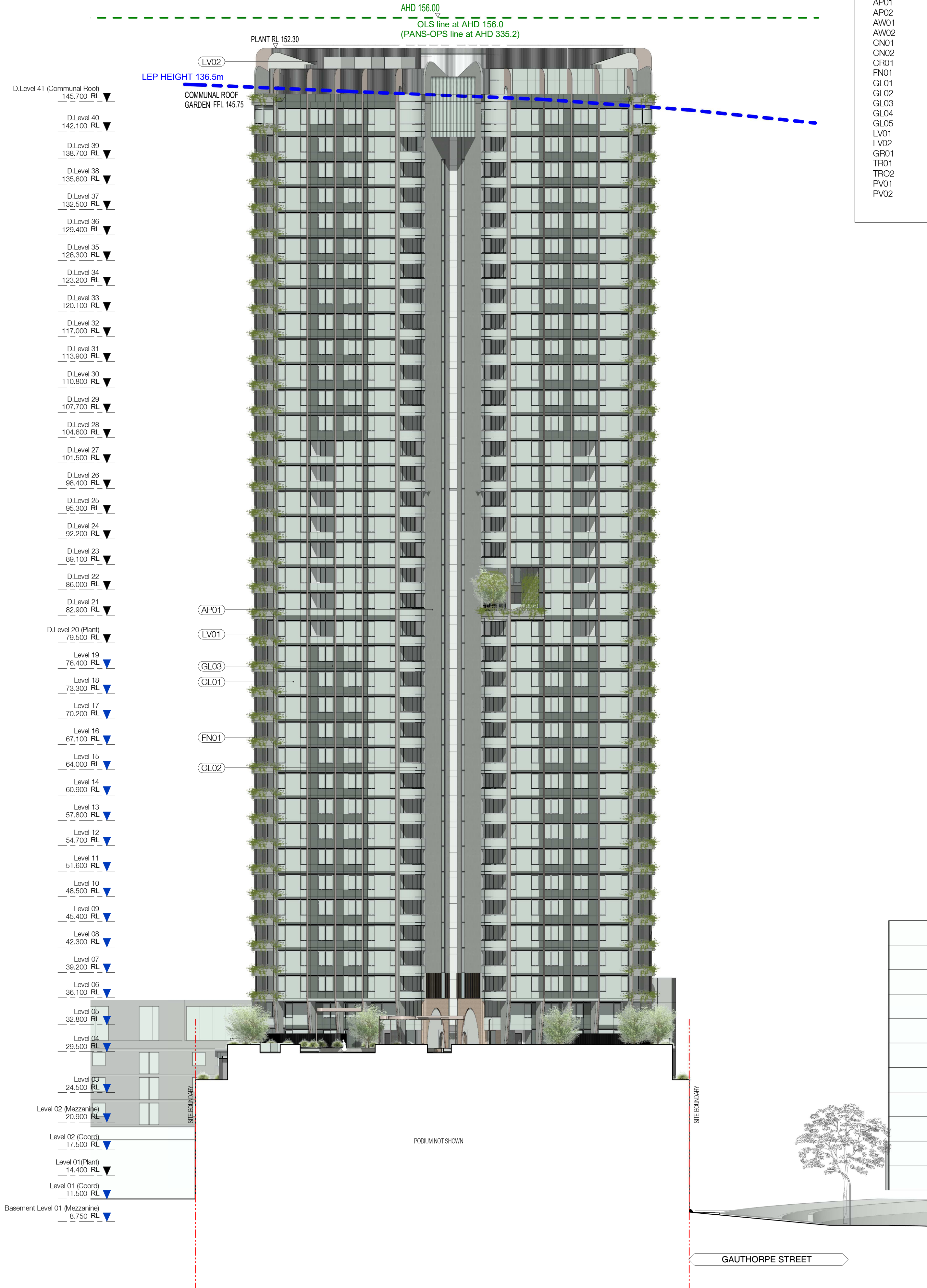
1 Internal Elevation Tower D A-Q-0307 1 : 300
